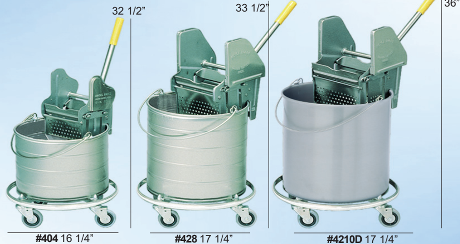
#404 16 1/4" #428 17 1/4" #4210D 17 1/4" 36" Bucket only 14" diam 10" height 14" diam 14" height 14" diam 16" height Gallon & Mop sizes 4-Gallon / 12-16 oz. 8-Gallon / 16-24 oz. 10-Gallon / 16-24 oz. Casters Four 3" rubber non-marking swivel casters attached with stainless steel tubing spider.
